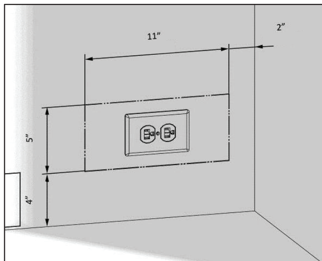
B. Location of the electrical wiring
